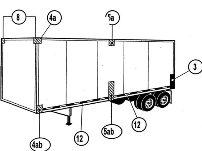
Figure 8- Semi-Trailer Illustration for§ 393.11
