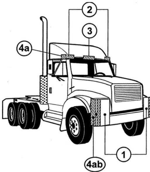
Figure 1 -Truck Tractor Illustration for§ 393.11 Annex 3
