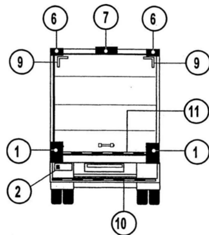
Figure 8- Semi-Trailer Illustration for§ 393.11
