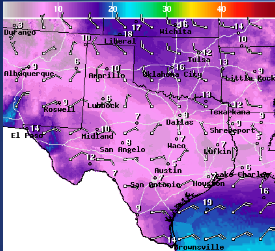
WindSpd(Kts) & WindDir For Fri Jan 27 2017 4PM EST (Fri Jan 27 2017 21Z)
