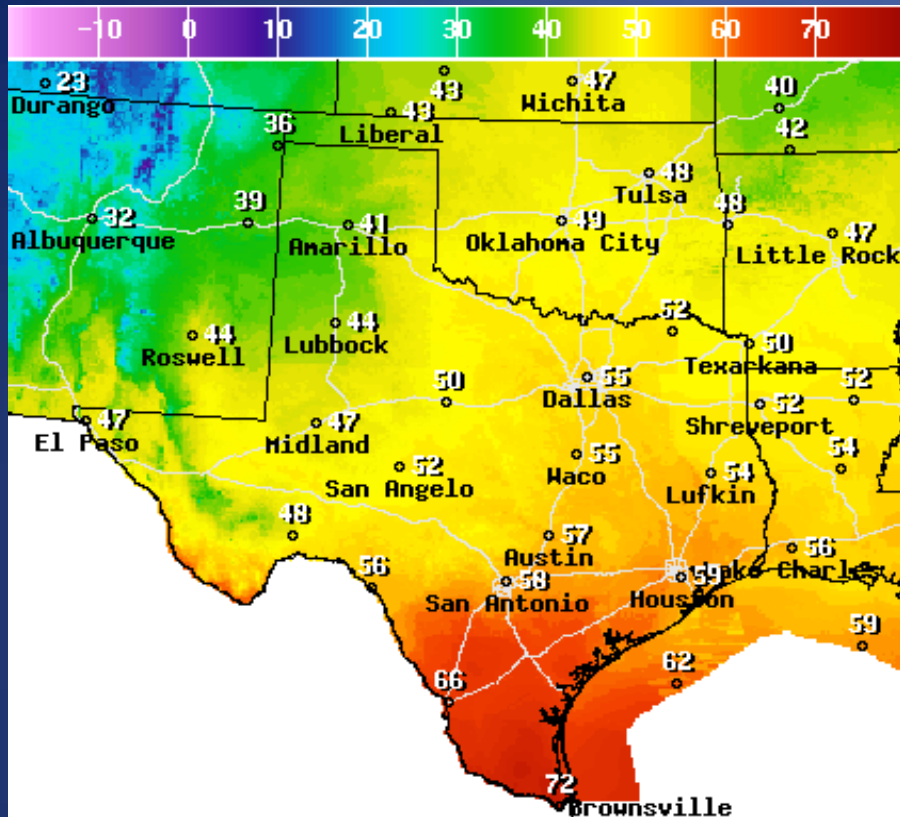
Temperature(F) For Fri Jan 27 2017 4PM EST (Fri Jan 27 2017 21Z)
